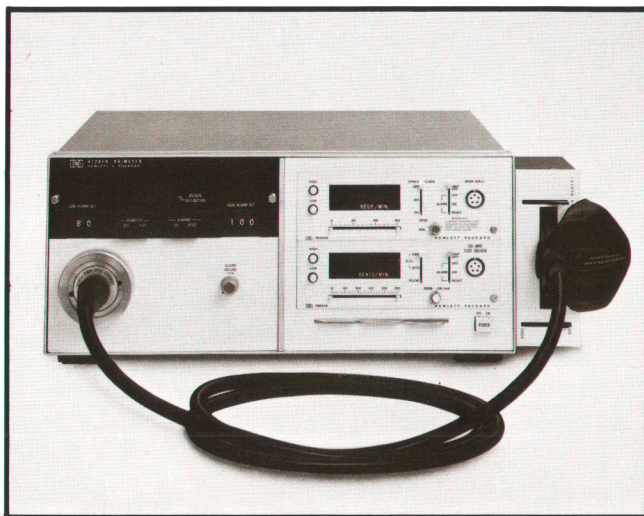
Fig. 7. Oximeter has space for optional patient-monitoring modules to give simultaneous measurements of heart rate, pressure, temperature, or respiration. Standardization cavity then mounts on the side of the instrument.
